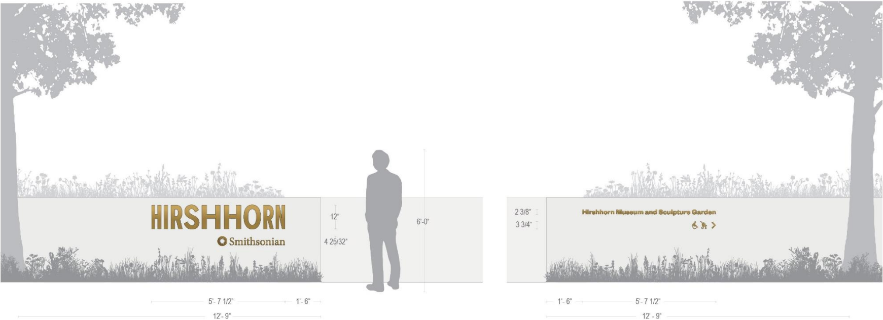
[1] North Overlook - North Elevation
