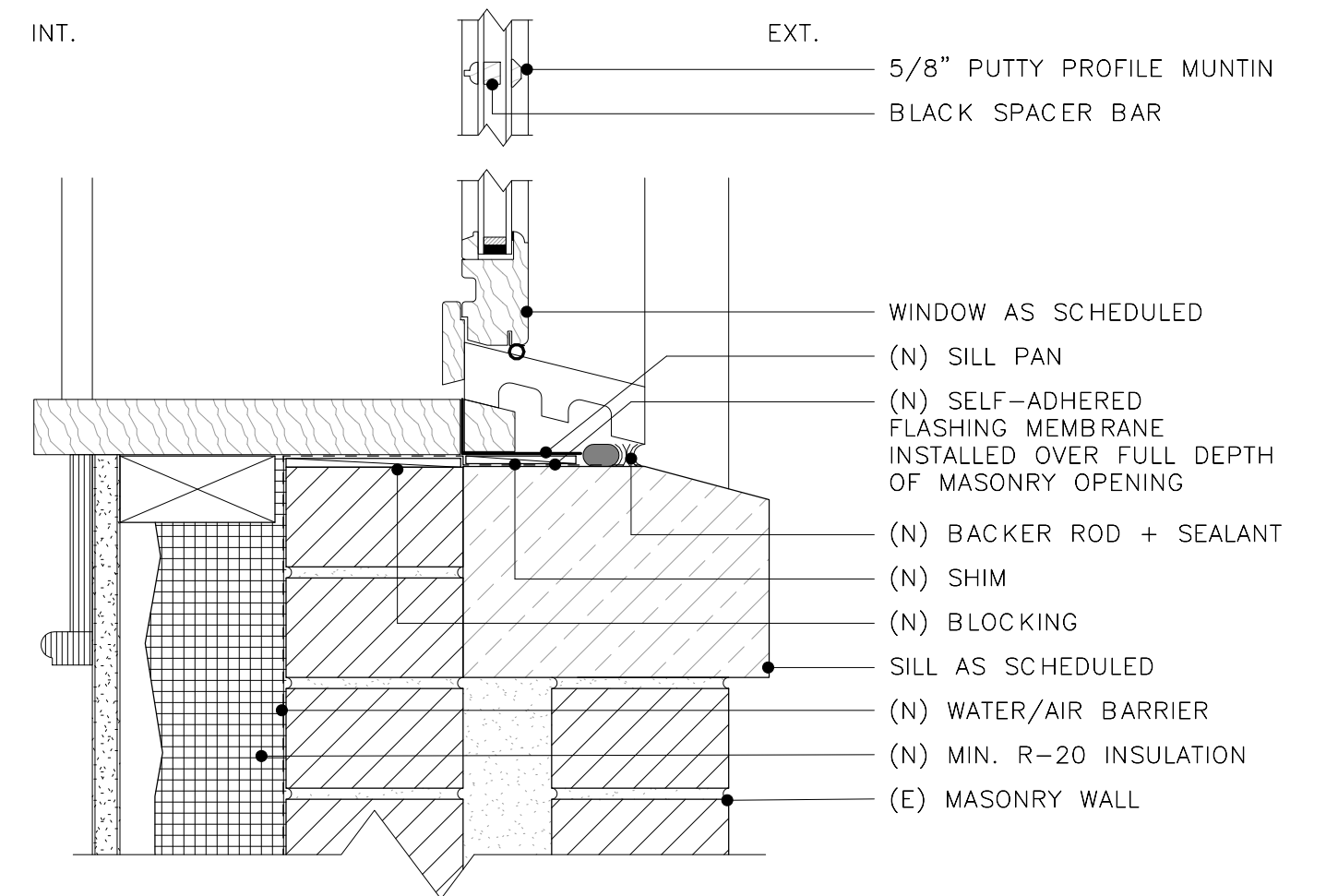
2 NEW WINDOW - JAMB 3" = 1'-0"
