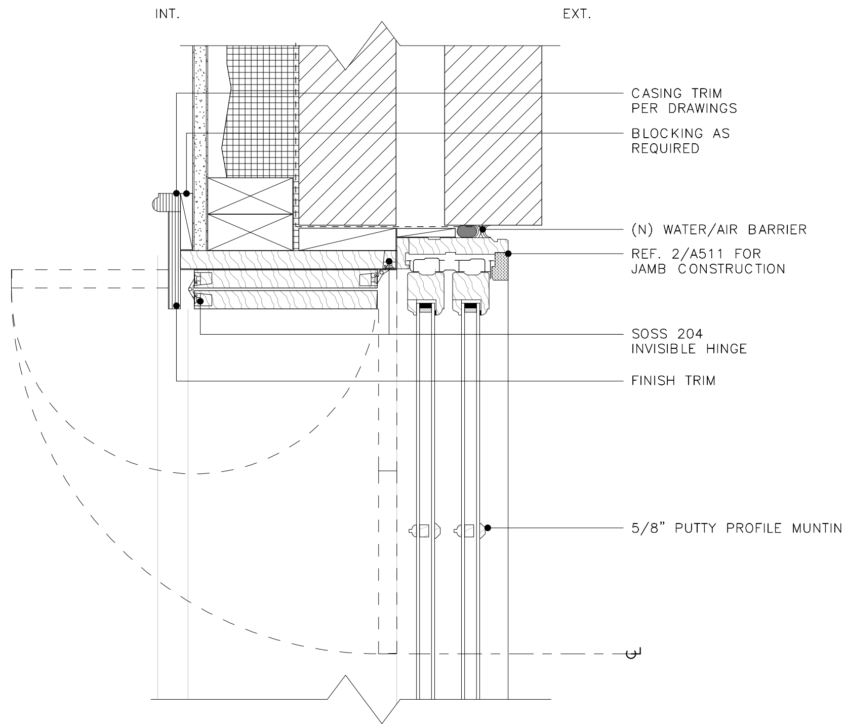
8 NEW WINDOW - JAMB WITH SHUTTERS 3" = 1'-0"
