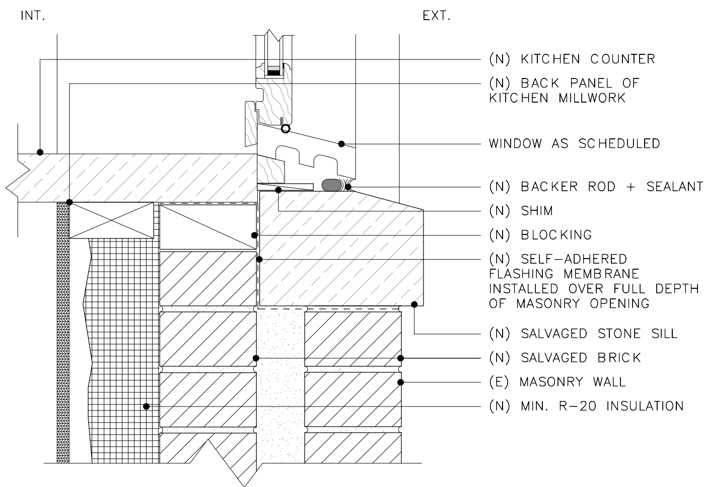
7 NEW WINDOW - RAISED SILL 3" = 1'-0"
