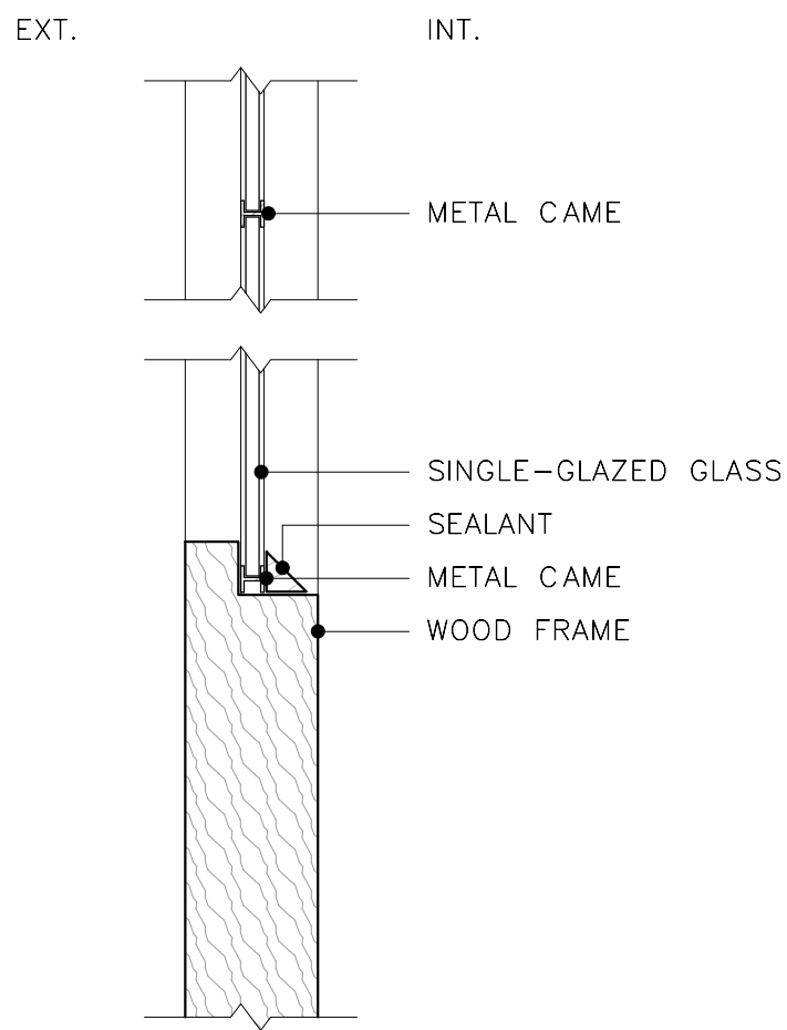
5 REFURBISHED WINDOW - LEADED LIGHT
