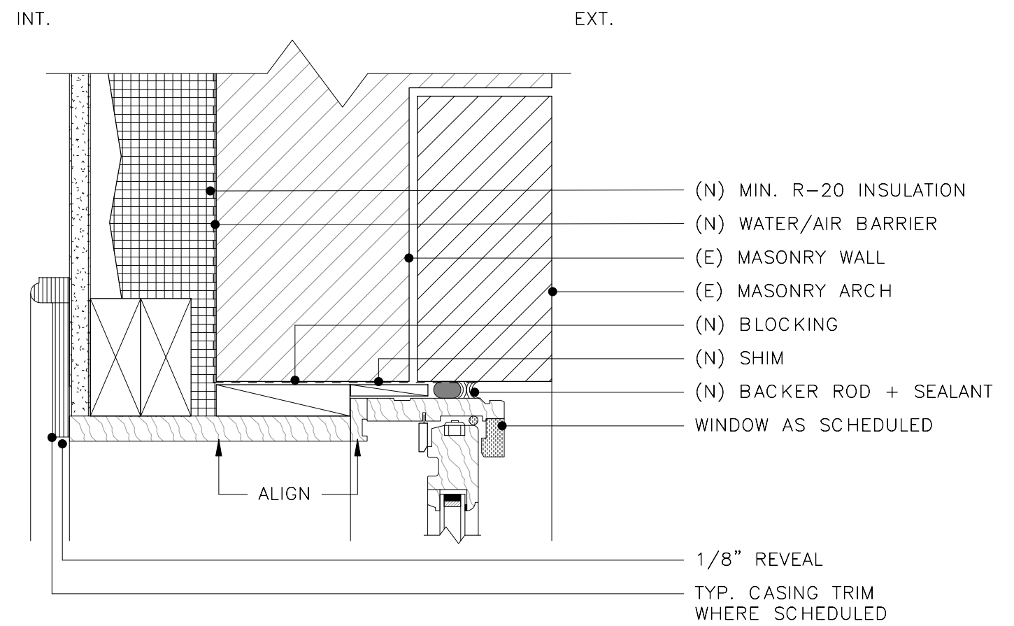
3 NEW WINDOW - HEAD 3" = 1'-0"
