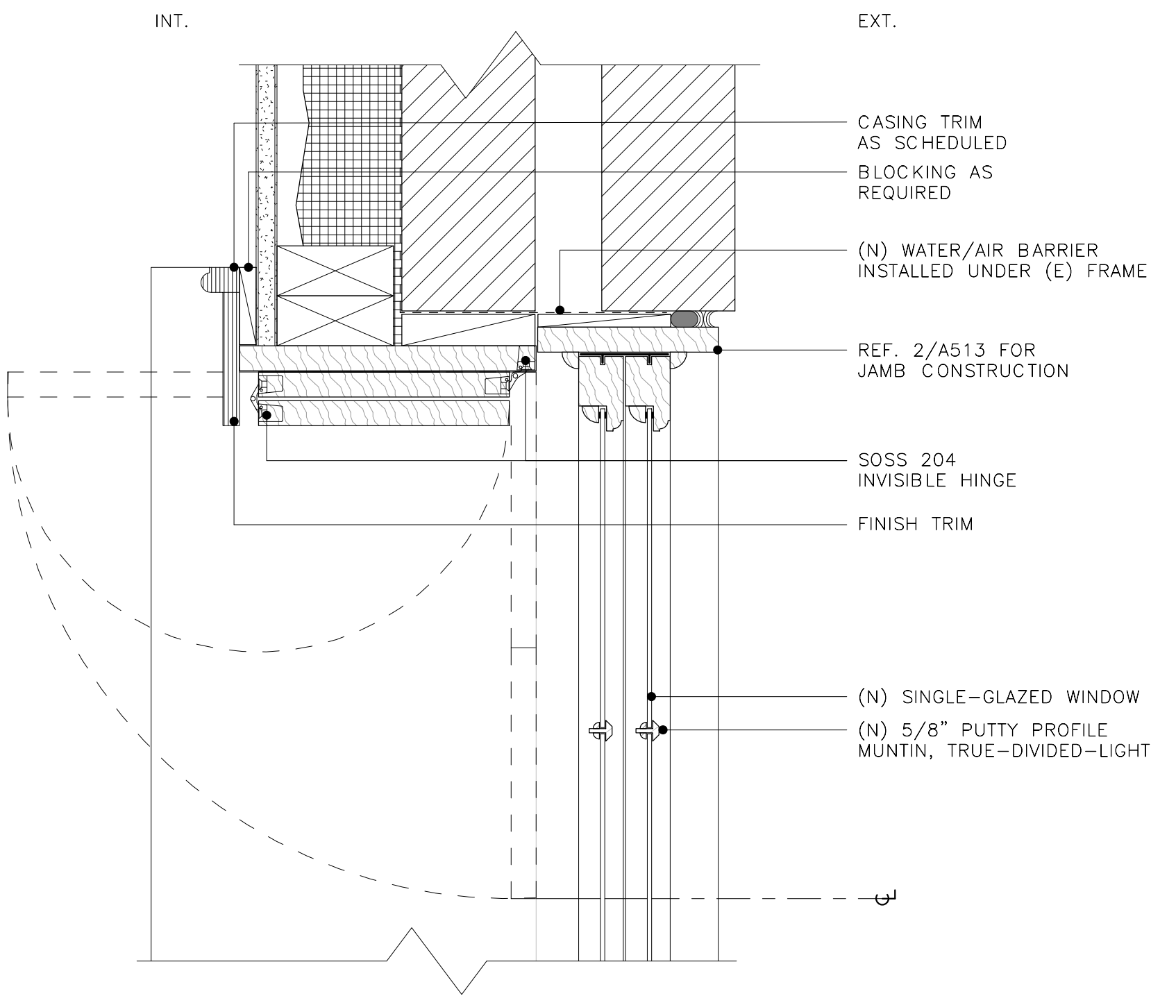
4 REFURBISHED WINDOW - JAMB WITH SHUTTERS
