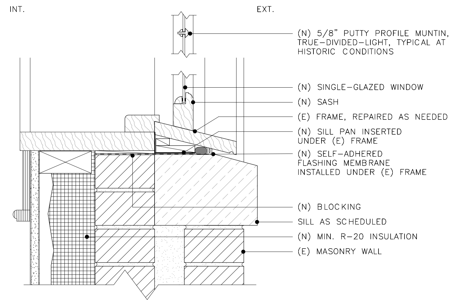
1 REFURBISHED WINDOW - SILL
