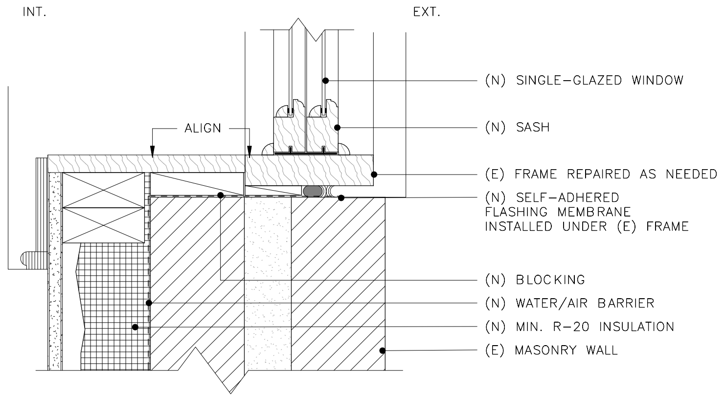
2 REFURBISHED WINDOW - JAMB
