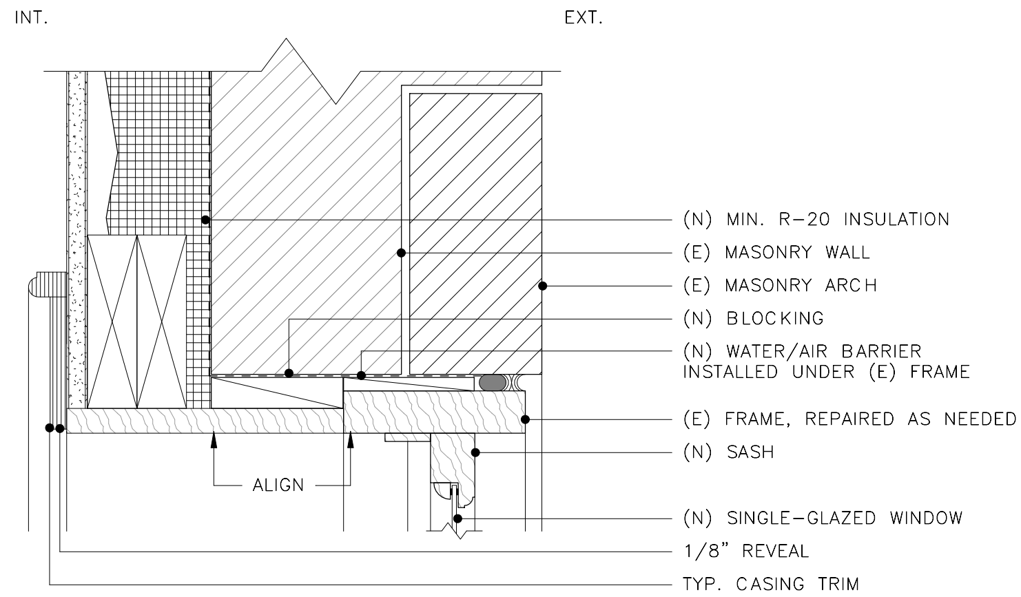
3 REFURBISHED WINDOW - HEAD
