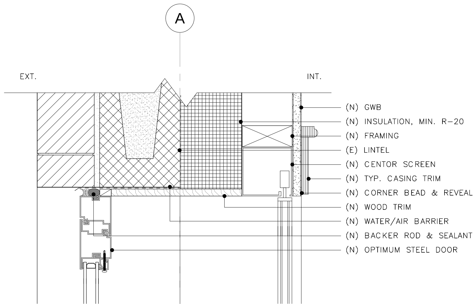
6 GARDEN DOOR - HEAD 3" = 1'-0"
