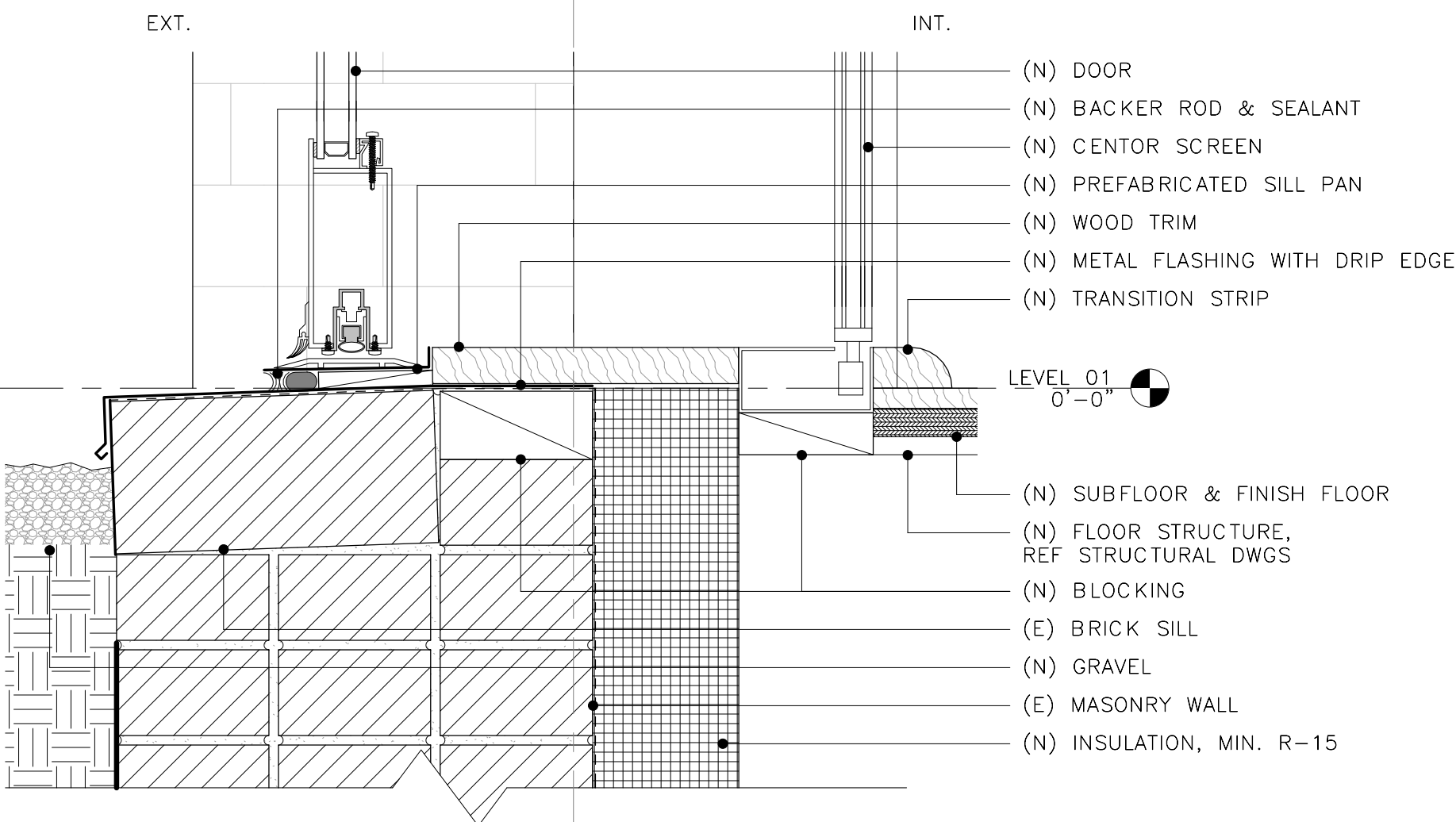
5 GARDEN DOOR - JAMB 3" = 1'-0"
