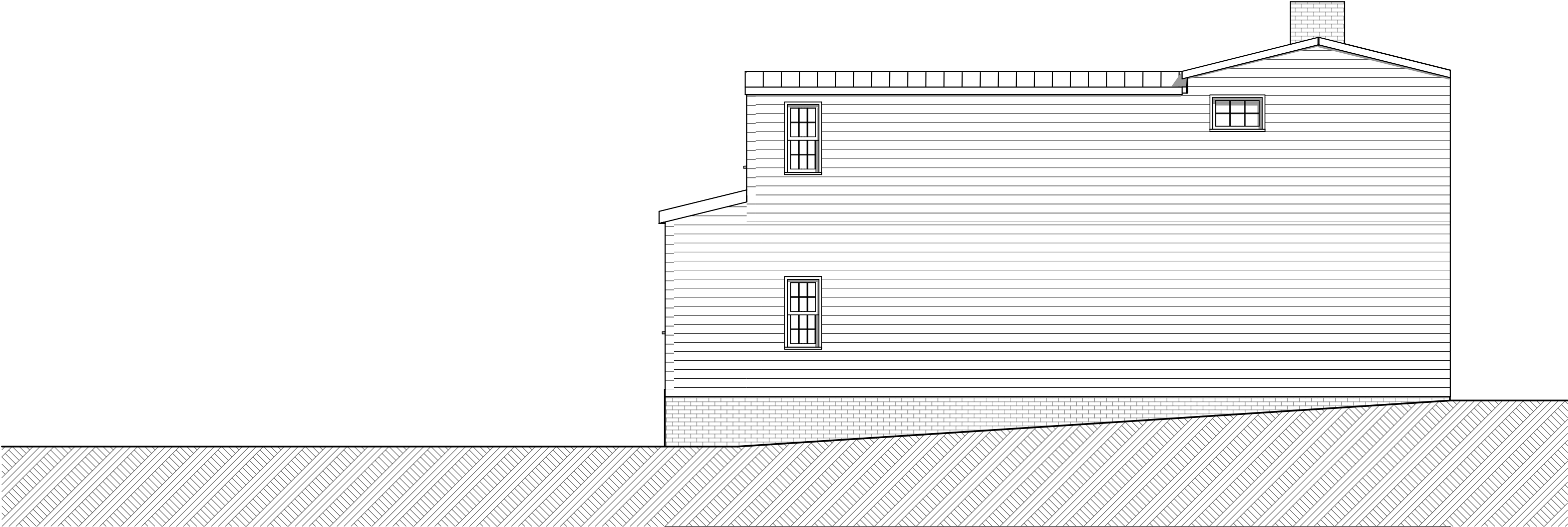
EAST ELEVATION
