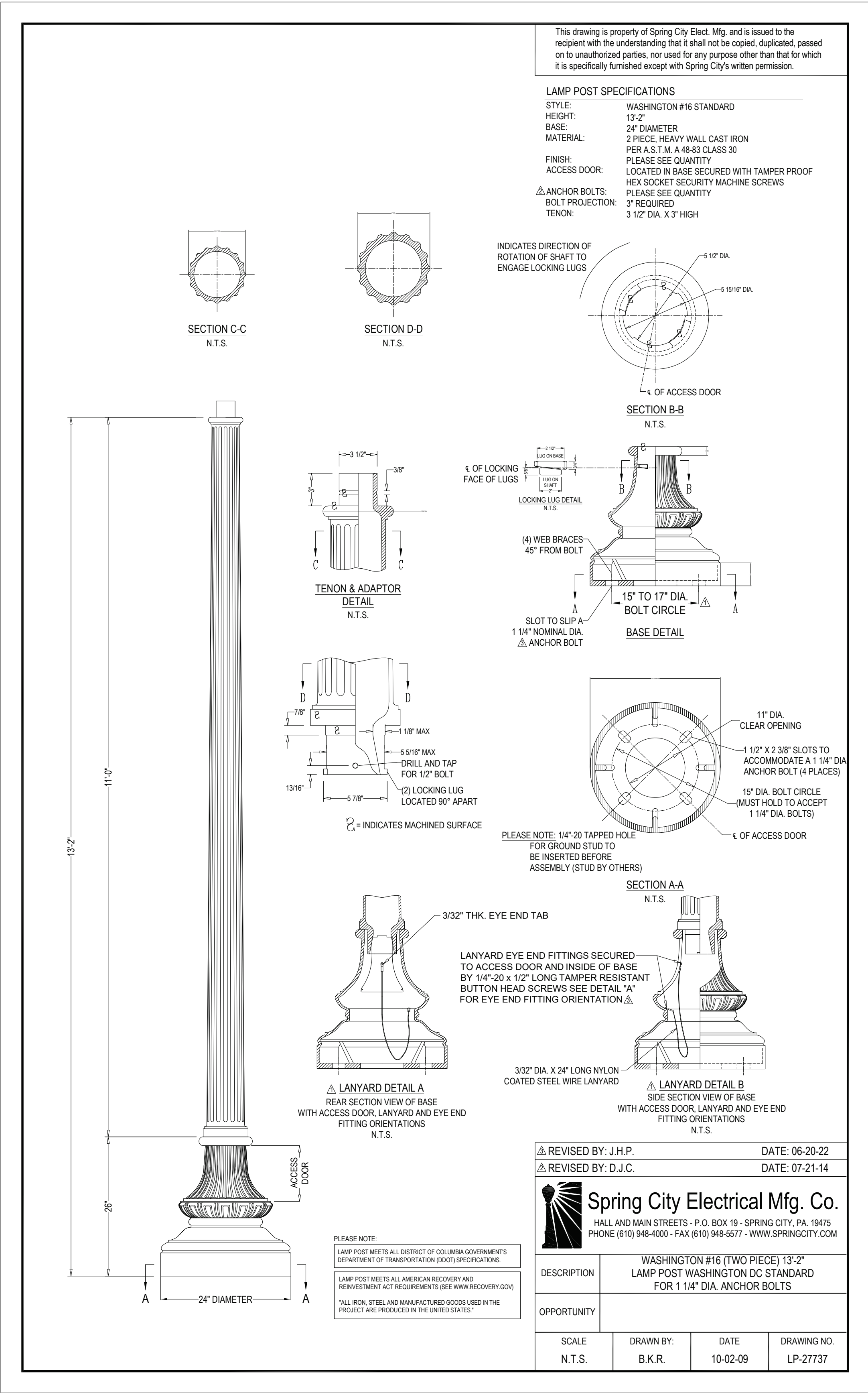
1 DDOT #16 POLE
