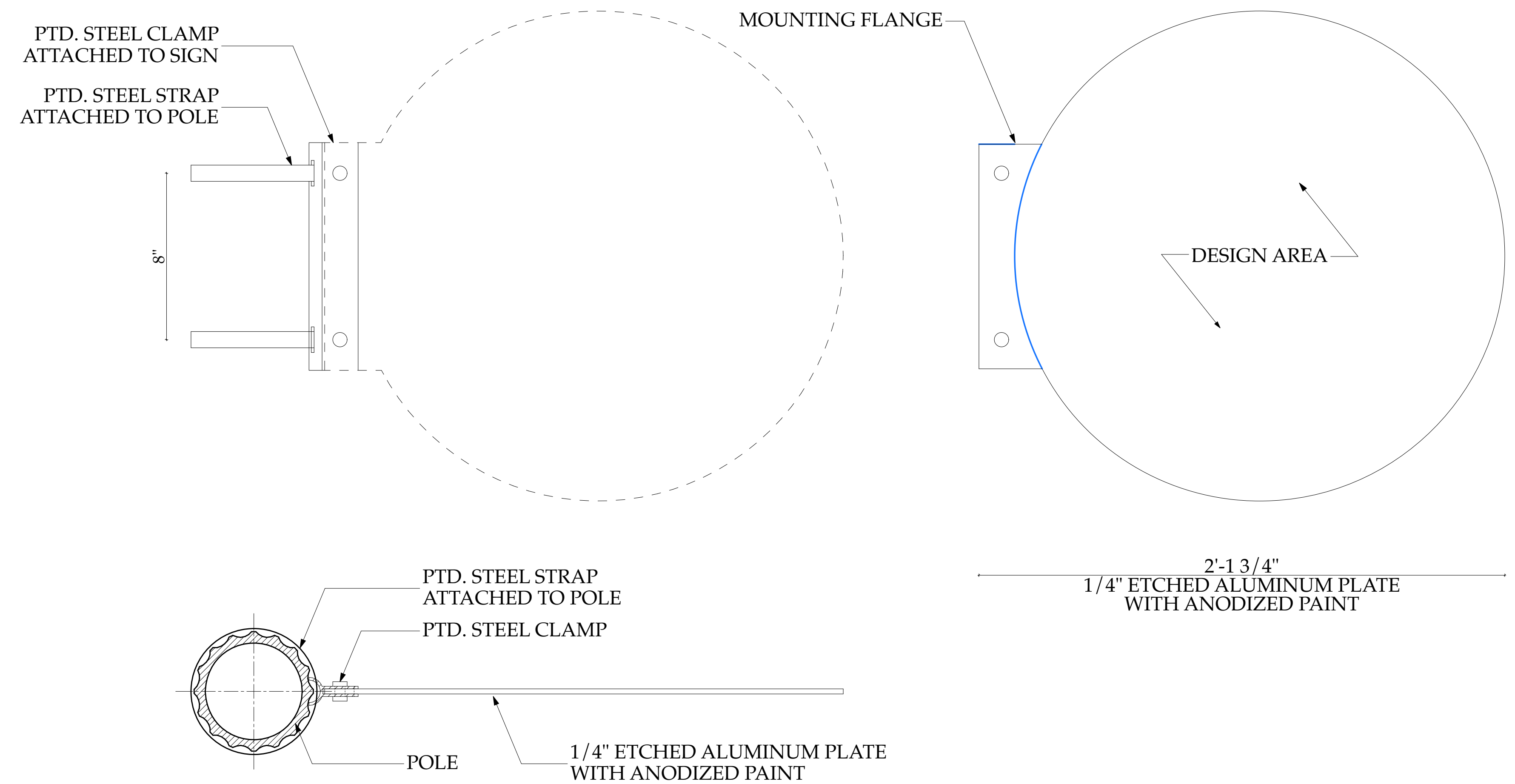
2 BRACKET ELEVATION & PLAN DETAILS SCALE: 3" = 1'-0"
